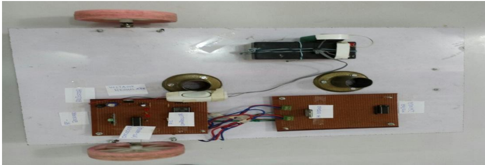
Figure 3 Different parts of receiver side that are R F receiver H-bridge, surge diodes, decoder, and regulator. Here H-bridge is used to drive the robot motors in desired direction, H-bridge is basically the combination of 4 relays (mean we can use H-Bridge instead of 4 Relays).the connection of each components is shown in circuit diagram.
