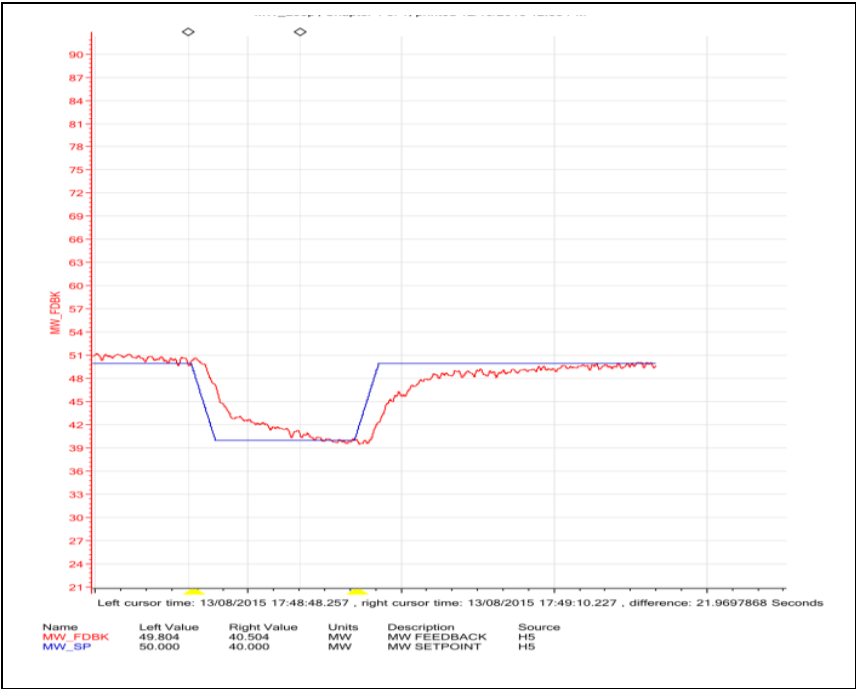
Fig 06: Step response of Megawatt
